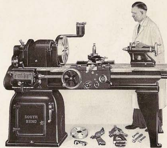
No. 192-C, 16" x 6' Underneath Belt Motor Driven Lathe $752.00
