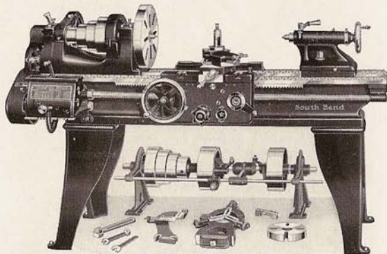
No. 92-C, 16" x 6' Quick Change Gear Lathe Including Regular Lathe Equipment..... $540.00
