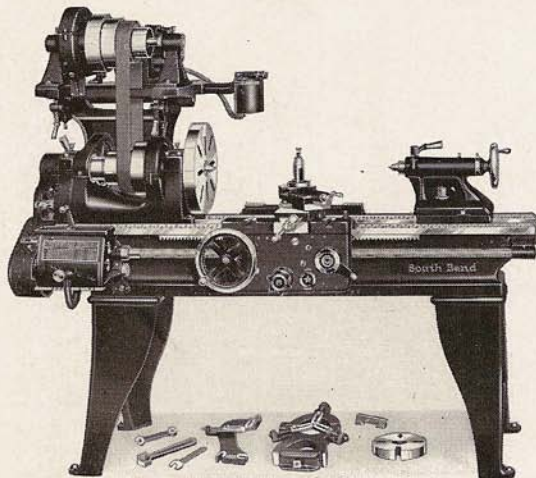
No. 392-C, 16" x 6' Silent-Motor Driven Lathe..... $682.00
