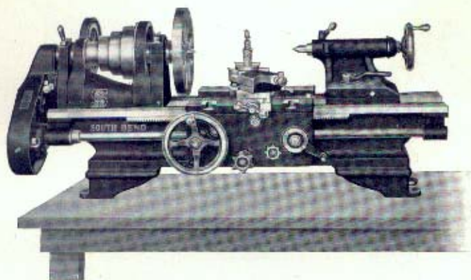
This is the Smallest Size Lathe We Build NO. 34—13-INCH SOUTH BEND LATHE
