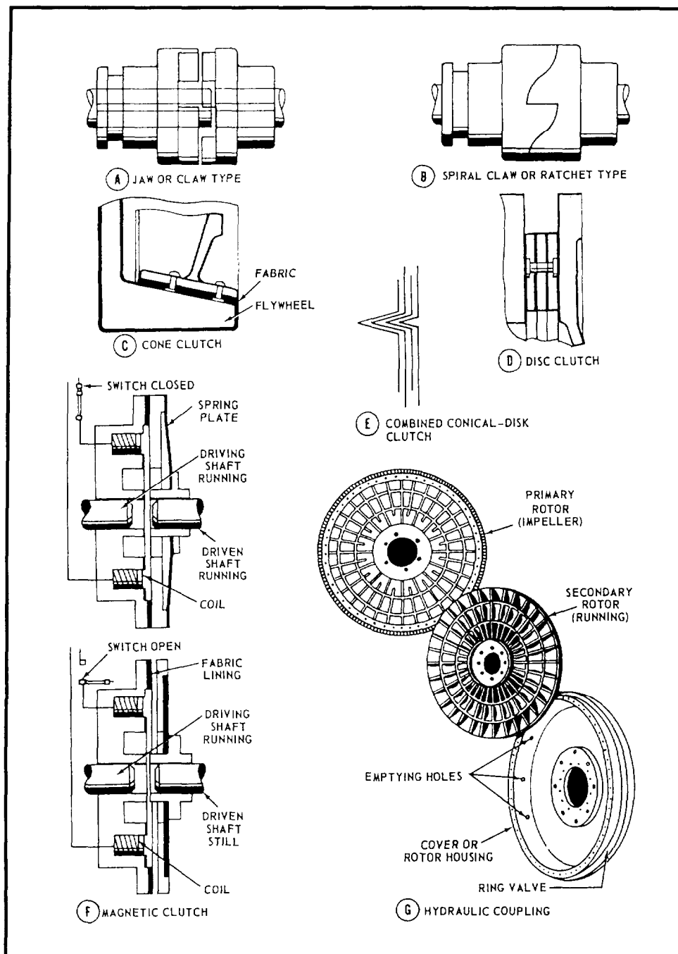
Figure 11-25.Types of clutches.
