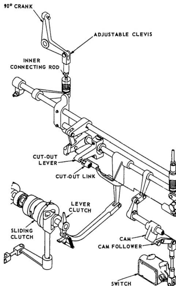
Figure 11-14.—Linkages.
