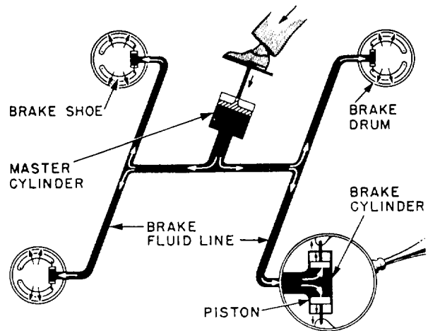
Figure 10-6.-Hydraulic brakes.
