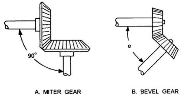
Figure 6-5.—Bevel gears.
