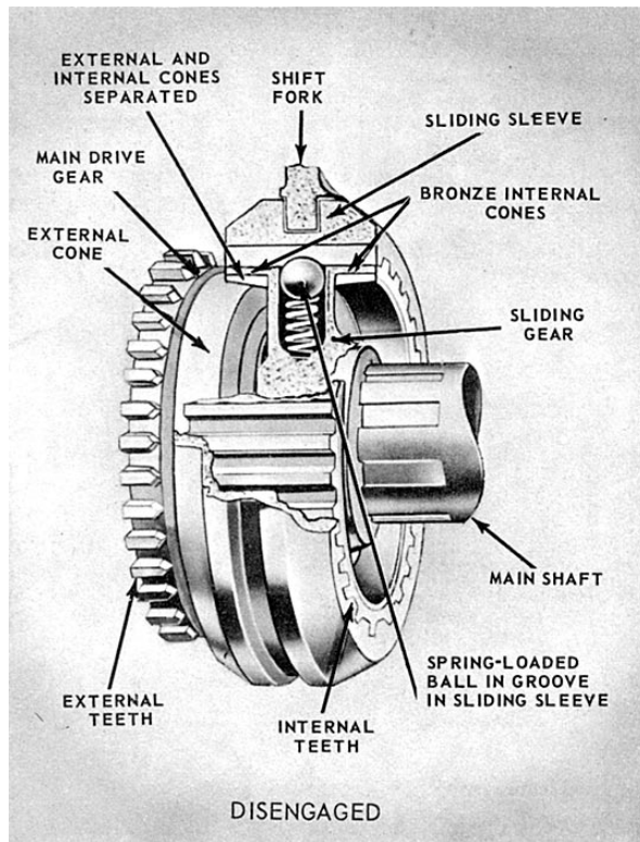
Figure 13-9.-Synchromesh clutch-disengaged and engaged.
