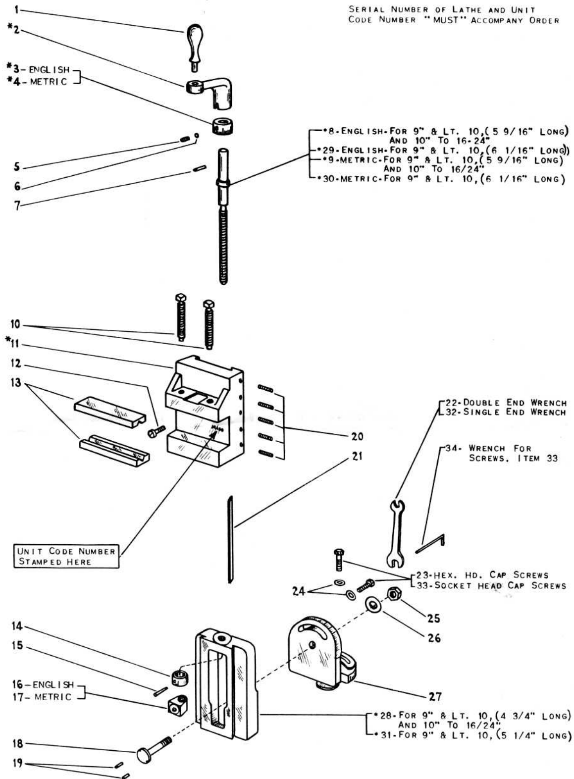
MILLING ATTACHMENT ENGLISH AND METRIC For 9", LT. 10, 10", 13", 14½", 16" & 16/24"
