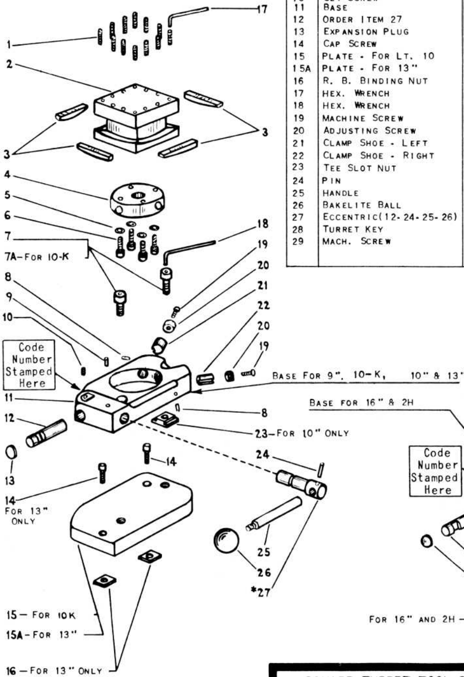
SQUARE TURRET TOOL BLOCK for Double Tool Cross Slide FOR 9", 10-K, 10", 13", 16" AND 2H
