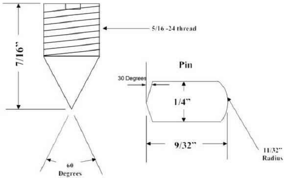
Set Screw
