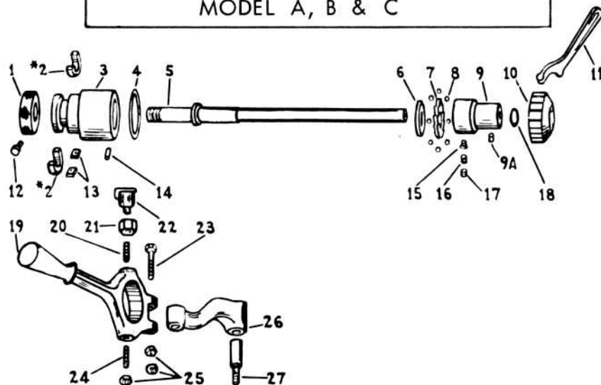
10-K HANDLEVER COLLET ATT. OLD STYLE MODEL A, B & C
